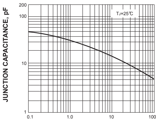
FIG. 5-TYPICAL JUNCTION CAPACITANCE
