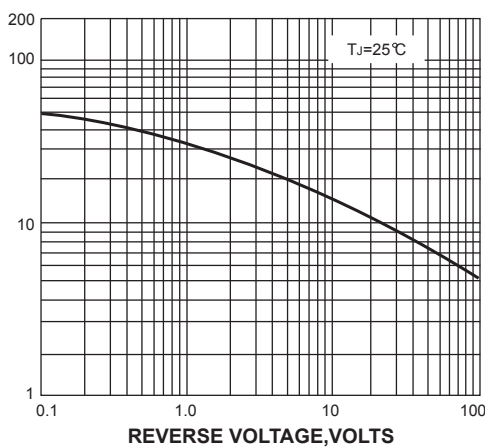
FIG. 5-TYPICAL JUNCTION CAPACITANCE
