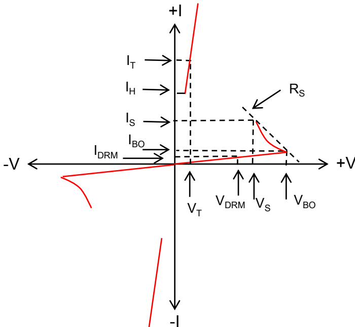
Figure 1. V-I Characteristics
